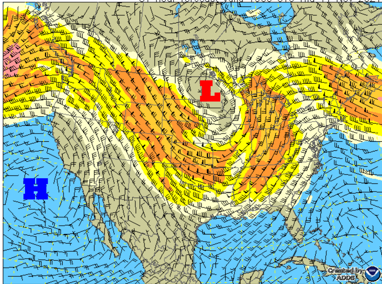
Wind speed (kts) at 15,000 MSL (575 mb)
